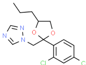
Propiconazole
